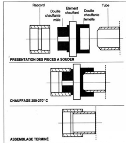
Figure 6 - Principe de soudage
